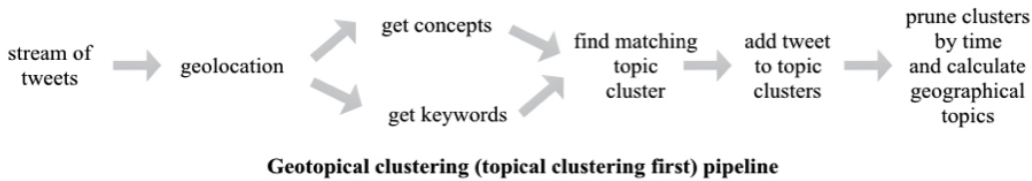
Fig. 1. GeoContext Pipeline
